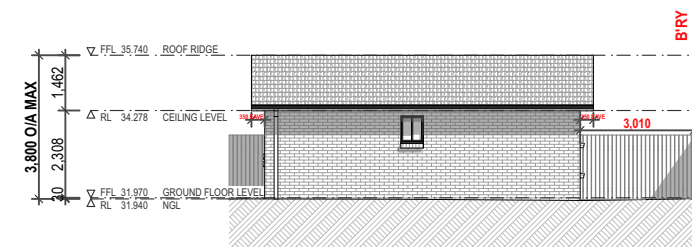
SIDE ELEVATION-SOUTH 1:200
