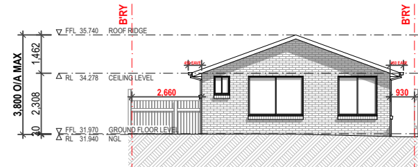
REAR ELEVATION-EAST 1:200
