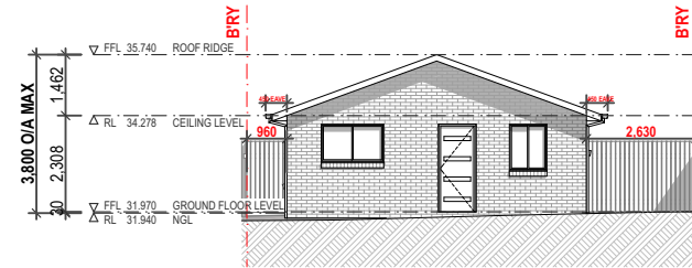
FRONT ELEVATION-WEST 1:200
