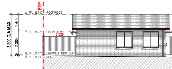
SIDE ELEVATION-NORTH 1:200
