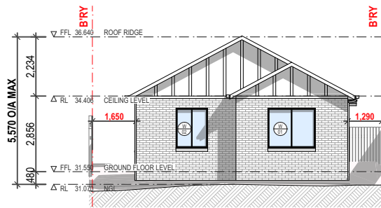
FRONT ELEVATION-WEST 1:200
