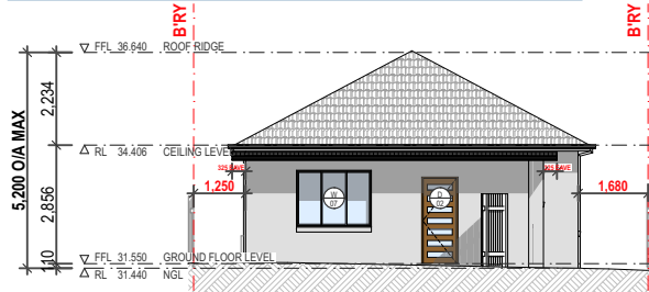
REAR ELEVATION-EAST 1:200
